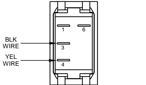
OLD VAC SWITCH 48B
