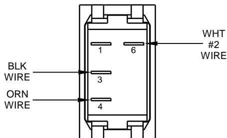
OLD SWITCH 48B
