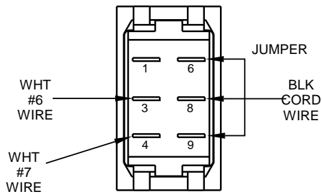
OLD SWITCH 48B
