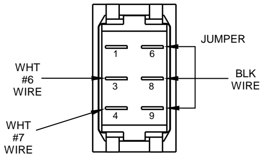
OLD SWITCH 50C
