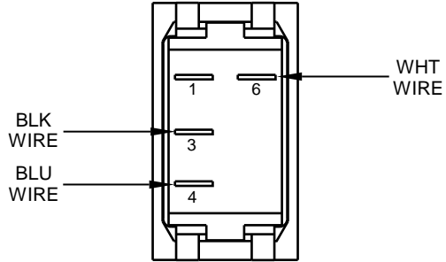
OLD PUMP SWITCH 48B
