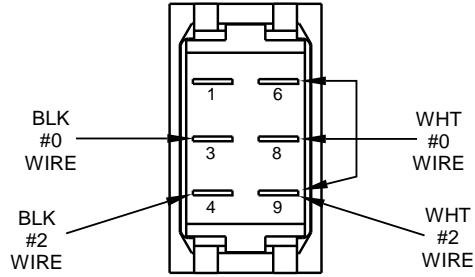
OLD 500 PSI PUMP SWITCH 50C
