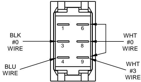
OLD VAC SWITCH 50C
