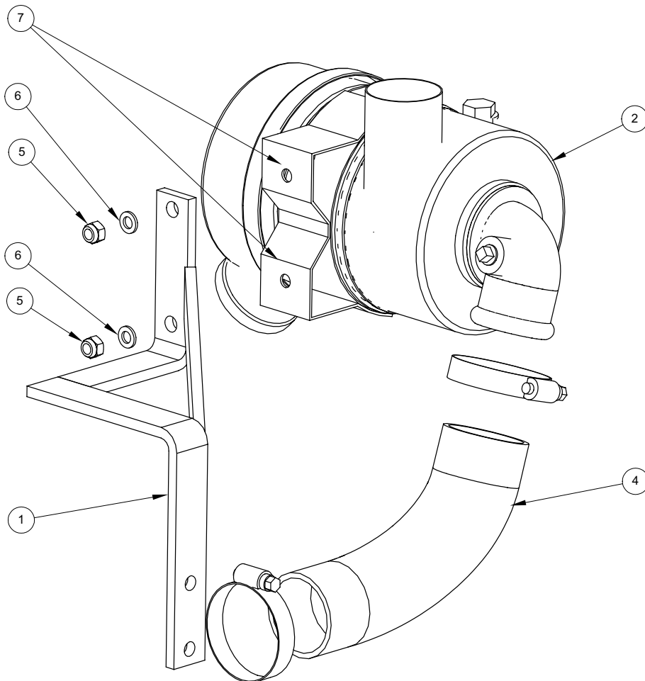
Figure 5-35 Air Cleaner Assembly CTS 450 Diesel C-5879 Rev -
