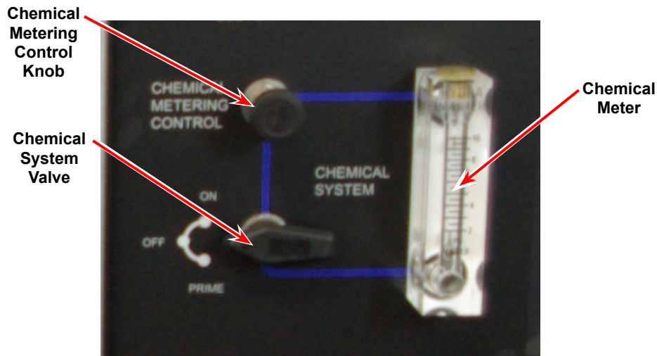
Figure 4. TITAN 425 Chemical System Control and Metering
