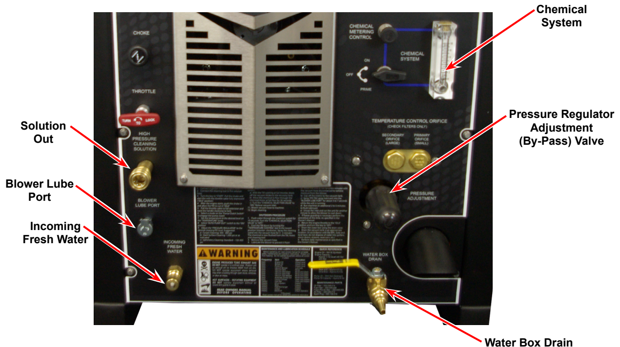
Figure 3. TITAN 425 Lower Dash Assembly
