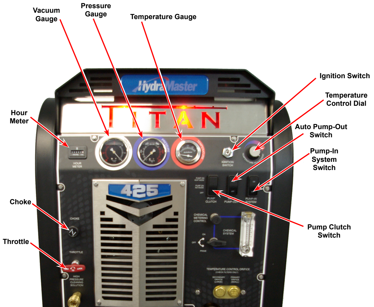
Figure 2. TITAN 425 Upper Dash Assembly
