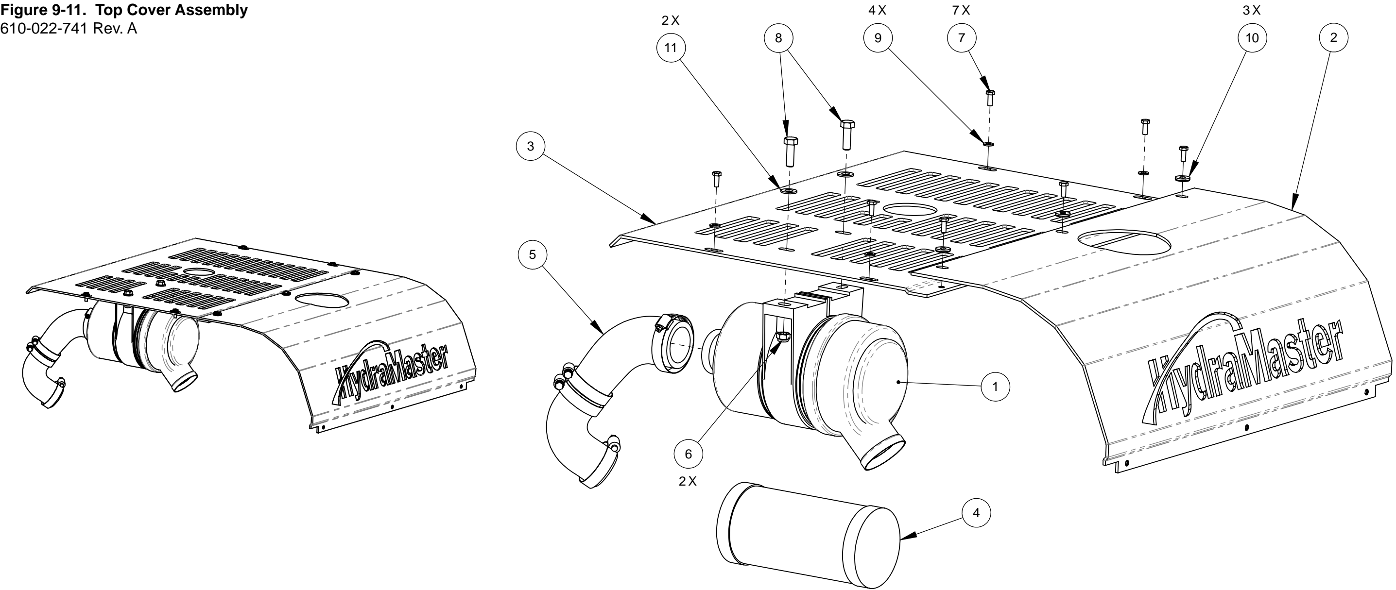
Top Cover Assembly Parts List
