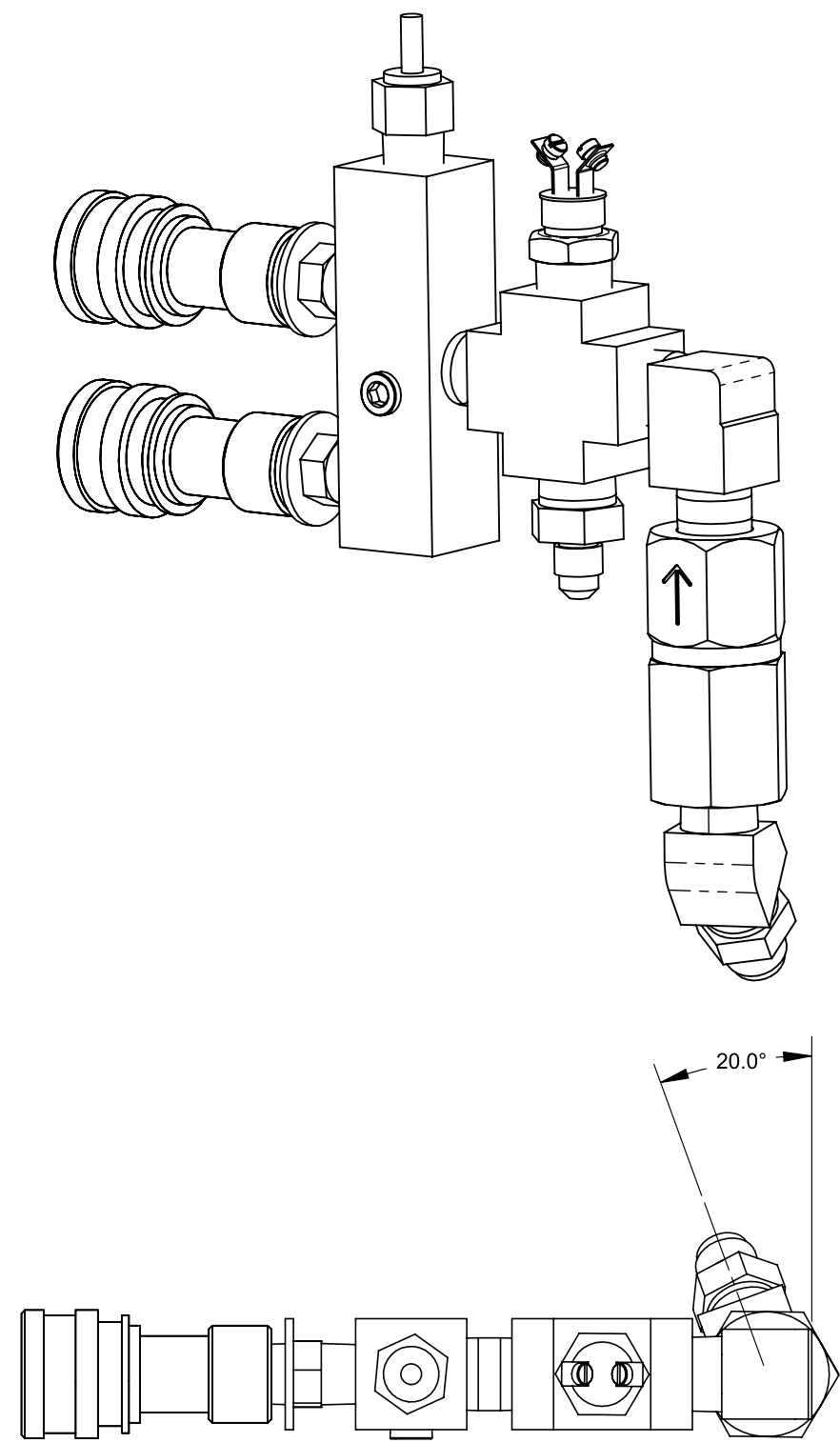
Figure 9-39. Hi Pressure Manifold Assembly 610-008-741 Rev. B
