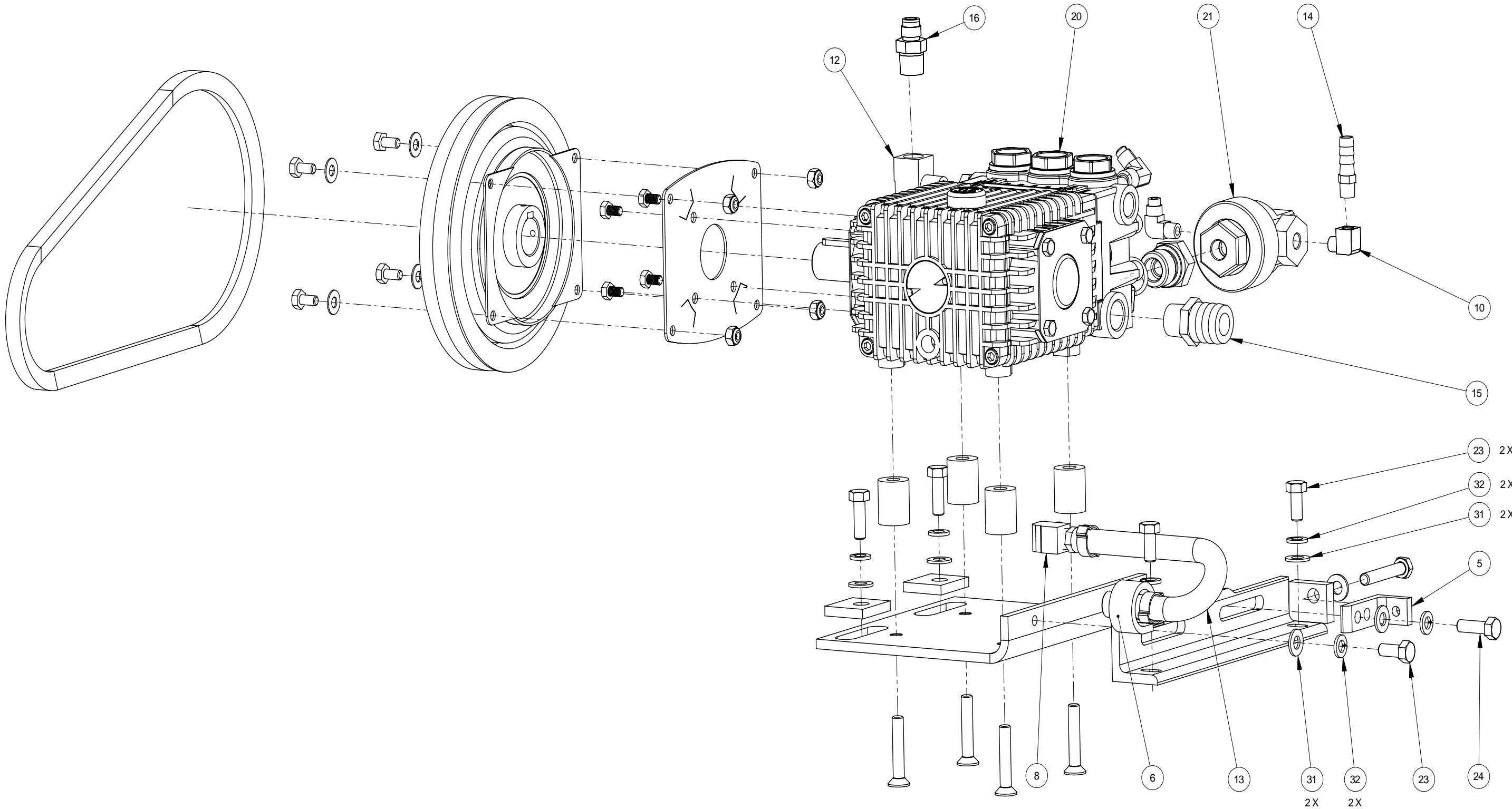
Figure 9-19. Pump Assembly - View 2 of 2 610-007-741 Rev. B
