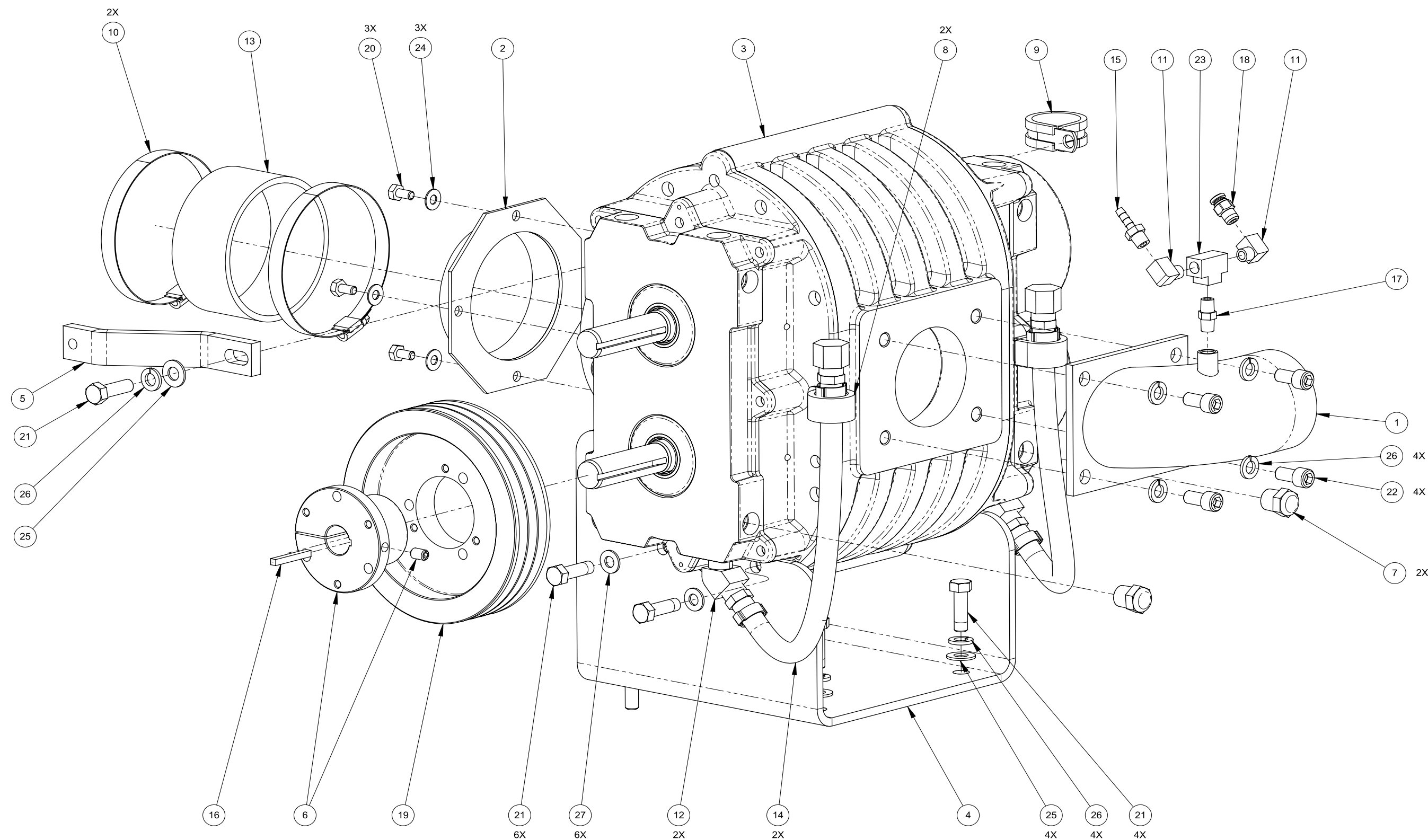
Figure 9-16. Blower Assembly 610-002-741 Rev. F
