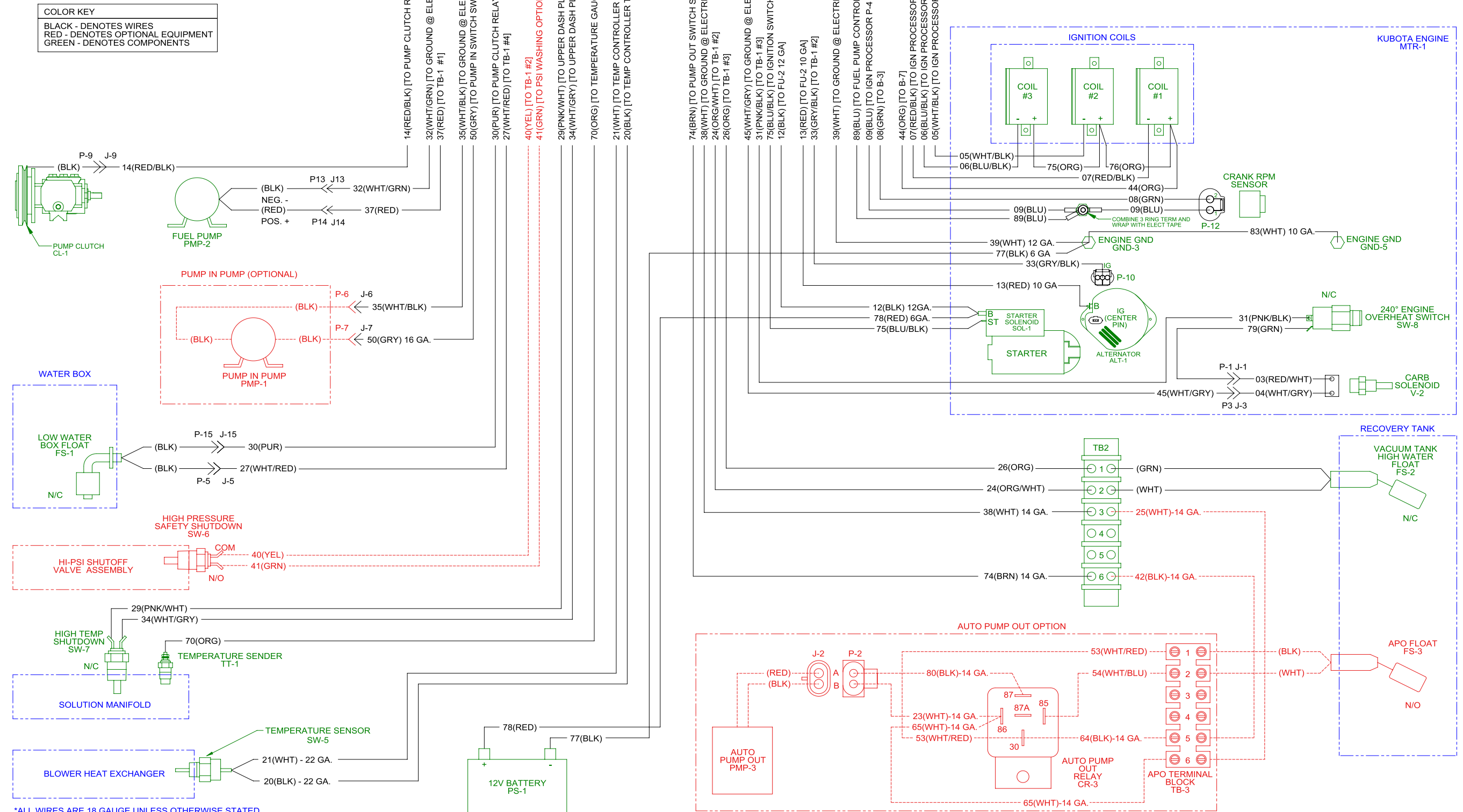
Figure 7-4. Wiring Diagram - View 3 of 3 000-179-022 Rev. G
