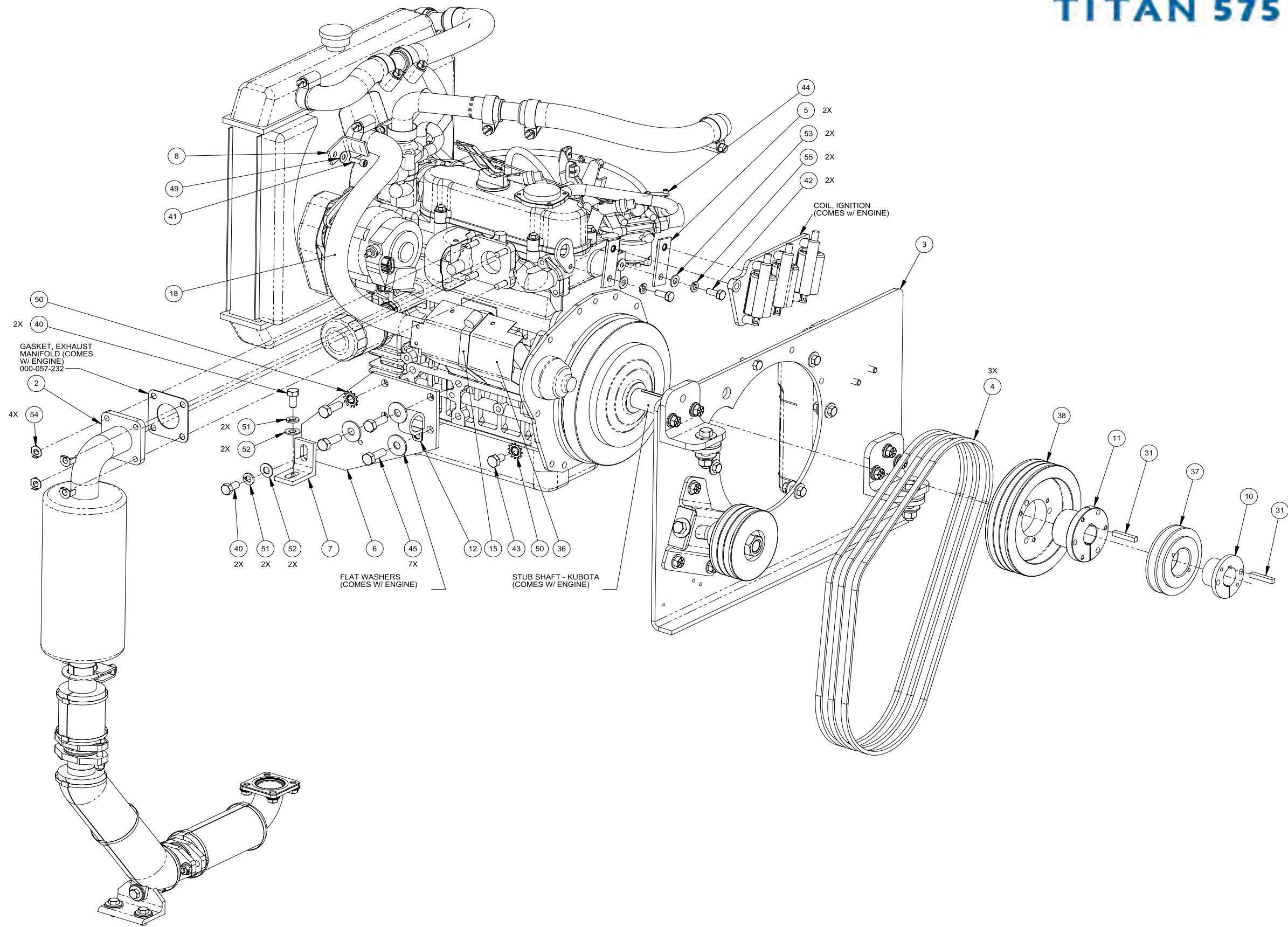
Figure 9-6. Engine Assembly - View 1 of 4 610-004-741 Rev. I
